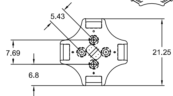
BASE DETAIL
